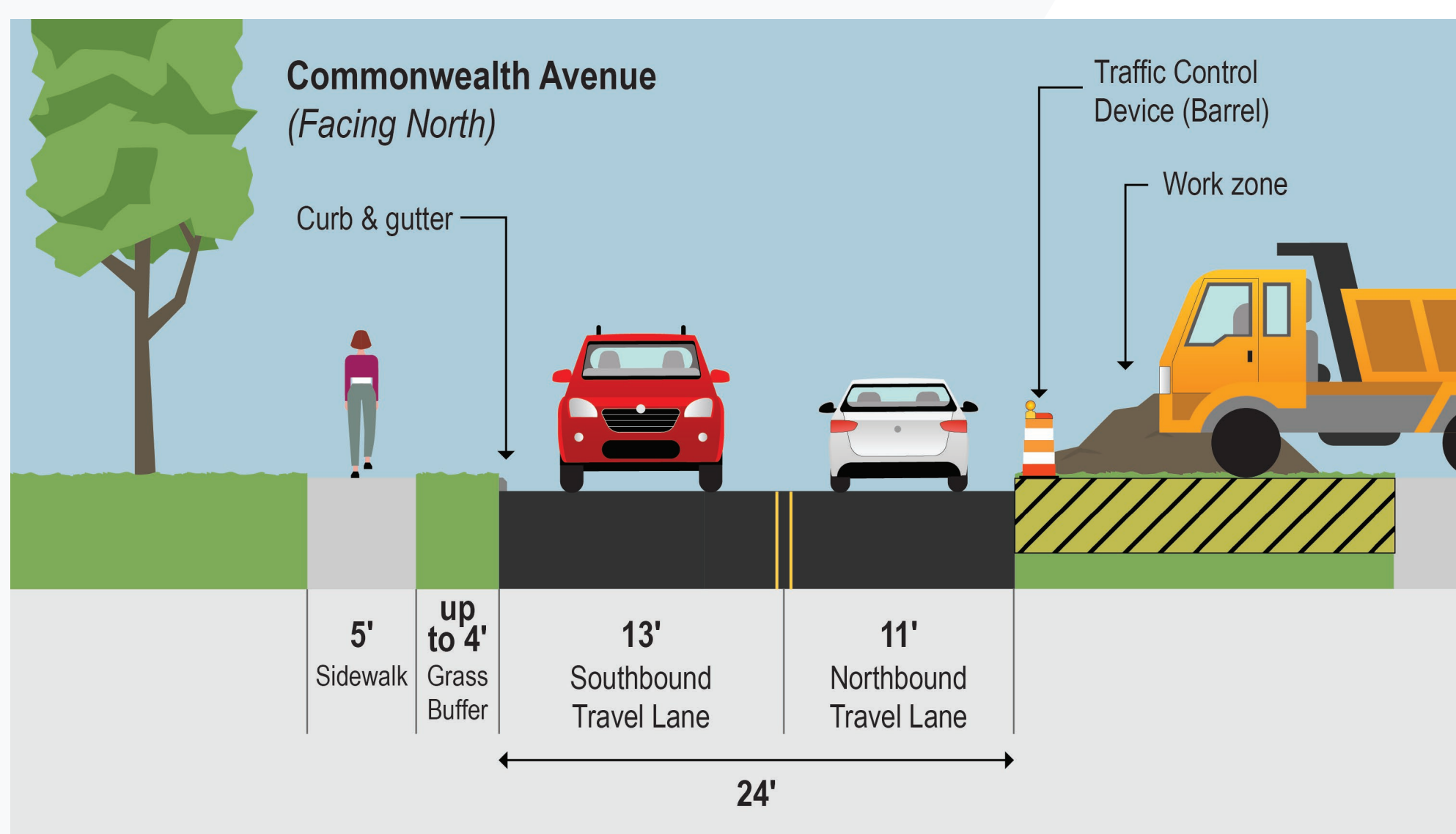
Two 7' x 8' box culverts will be installed on the east side of Commonwealth Ave
