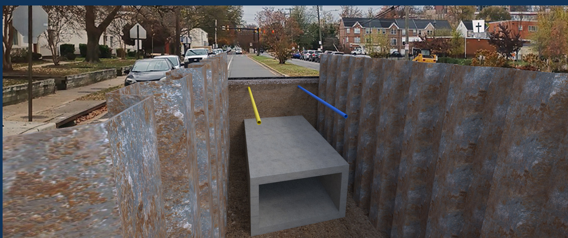
Similar construction in Richmond, VA (without open traffic lanes)
